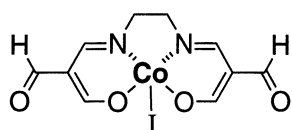
Fig. 8. The prototypal molecule for computations; iodo[ N,N' -bis(3-oxo-2-formylpropylidene)-ethylenediaminato]cobalt(III) (7).
