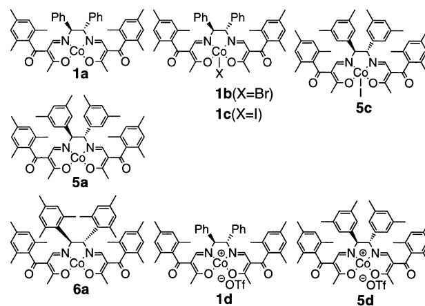
Fig. 2. Various 3-oxobutylideneaminato cobalt(II) and cobalt(III) complexes.
