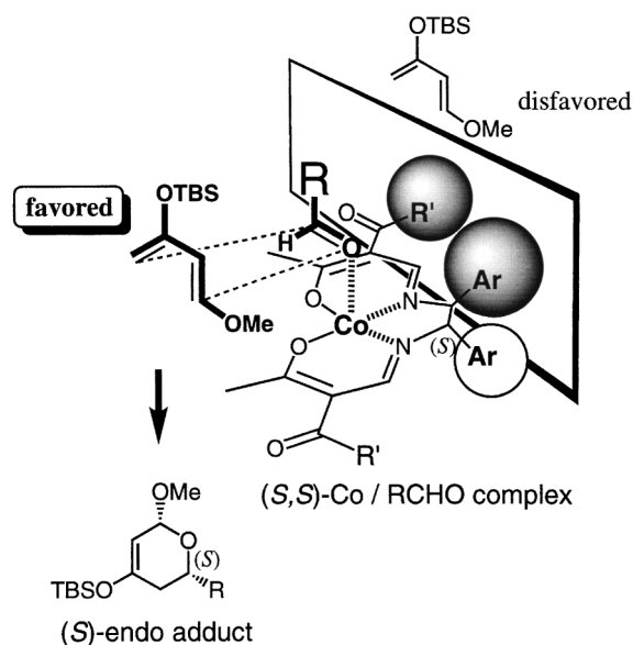
Fig. 7. Reasonable explanation for the endo-selection and the enantioselection in the hetero Diels-Alder reaction catalyzed by (S,S) -cobalt complex.
