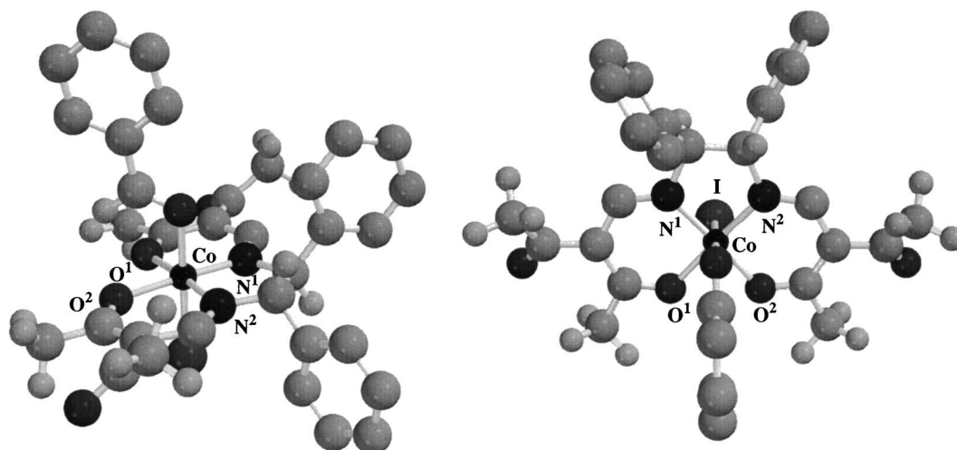
Fig. 6. The optimized structure of (S,S) -cobalt/PhCHO complex by semi-empirical method with Mac Spartan Pro (PM3(tm)). Side view (left) and top view (right).
