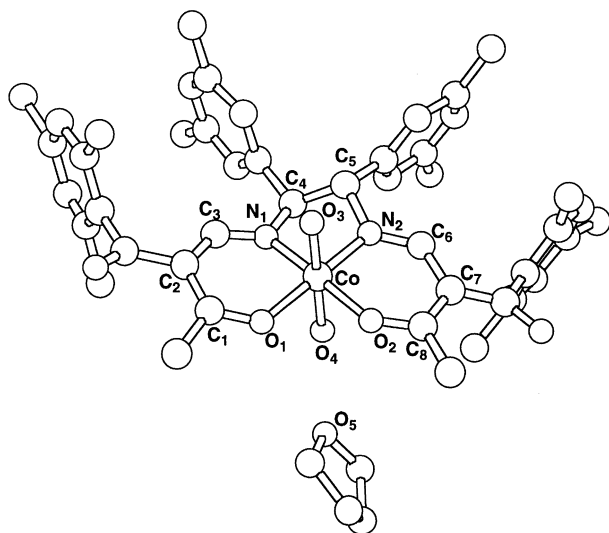
Fig. 3. Crystal structure of {(1 S ,2 S )-1,2-bis(3,5-dimethylphenyl)- N,N' -bis[3-oxo-2-(2,4,6-trimethylbenzoyl)butylidene]ethylenediaminato}cobalt(III) trifluoromethanesulfonate dihydrate ( 5d ): Selected bond lengths (Å) and bond angles (°) are as follows: Co–O1, 1.899(7); Co–O2, 1.912(8); Co–N1, 1.864(8); Co–N2, 1.853(8); Co–O3, 1.939(8); Co–O4, 1.931(8); O1–Co–N2, 179.1(3); O2–Co–N1, 178.8(4); O1–Co–O2, 86.0(3); O1–Co–N1, 93.3(3); O2–Co–N2, 94.8(4); N1–Co–N2, 85.8(4); O1–Co–O4, 89.4(3); O2–Co–O4, 88.6(3); O4–Co–N1, 90.5(3); O4–Co–N2, 90.2(4); (Two molecules exist in each unit cell, and one of them and – OSO 2 CF 3 ion were omitted for clarity).
