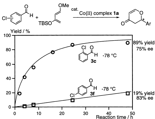
Fig. 4. Time-course of hetero Diels–Alder reaction for o - and p -chlorobenzaldehydes.
